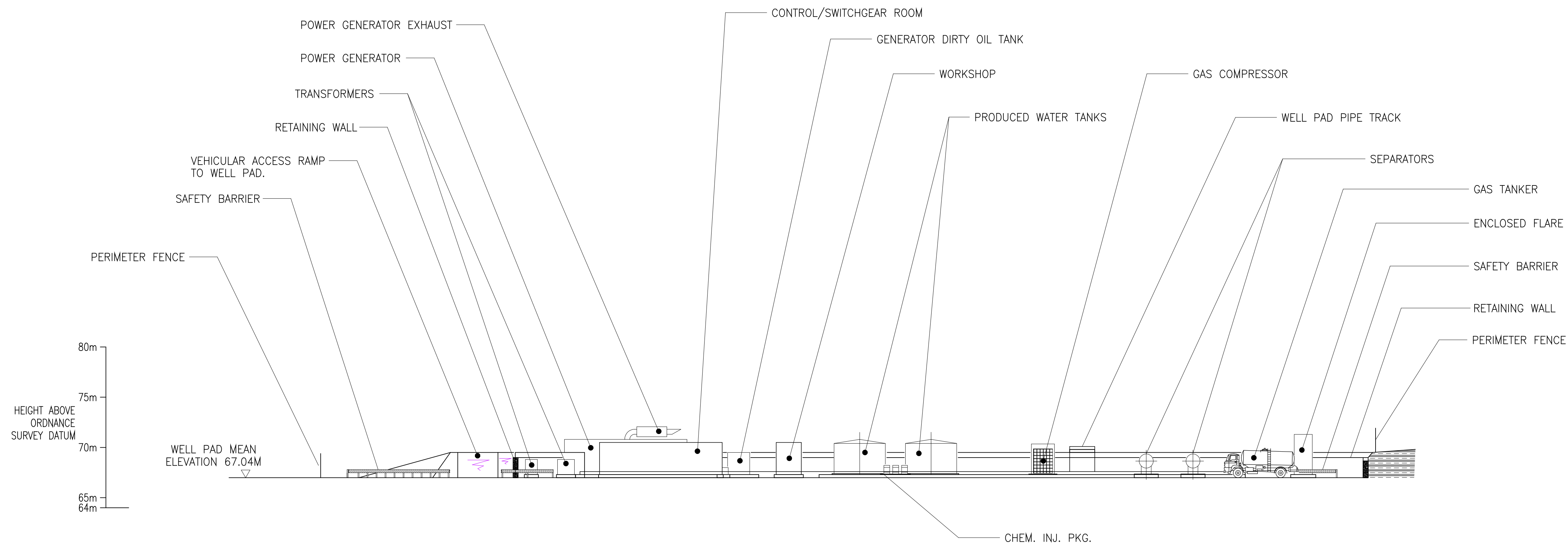
ILLUSTRATIVE SECTION D-D THROUGH PROCESS FACILITIES LOOKING WEST
